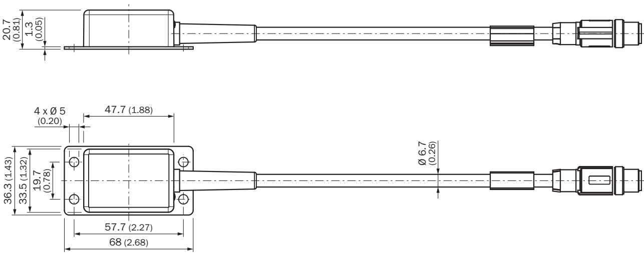
Dimensions in mm (inch)
