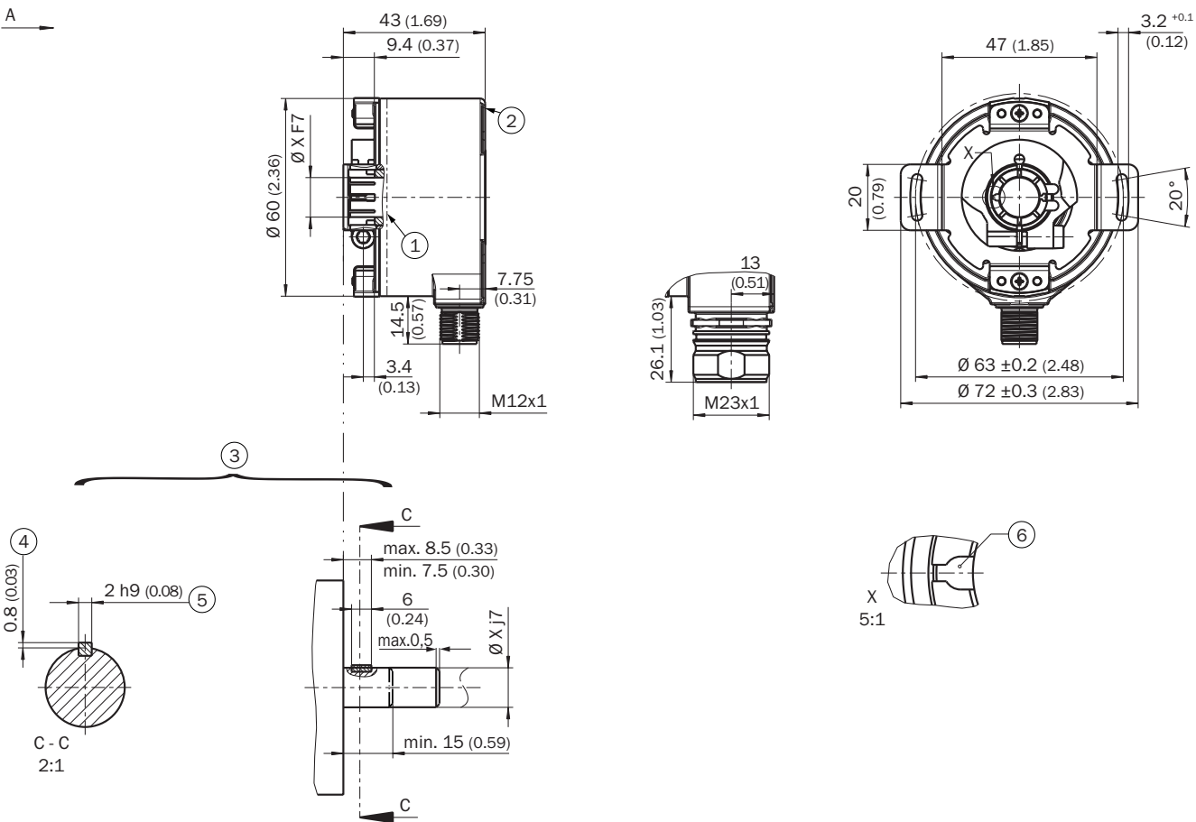
Dimensional drawing Through hollow shaft, M12 and M23 radial male connector
