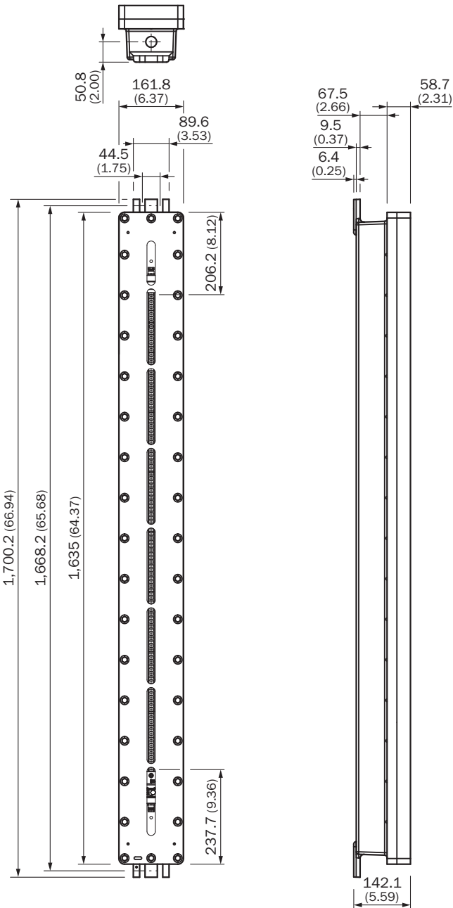
Dimensional drawing C4000 Select Ex, 1,200 mm
