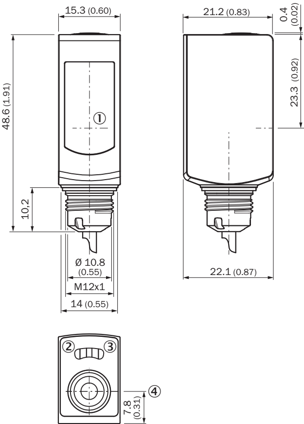
Dimensions in mm (inch)
