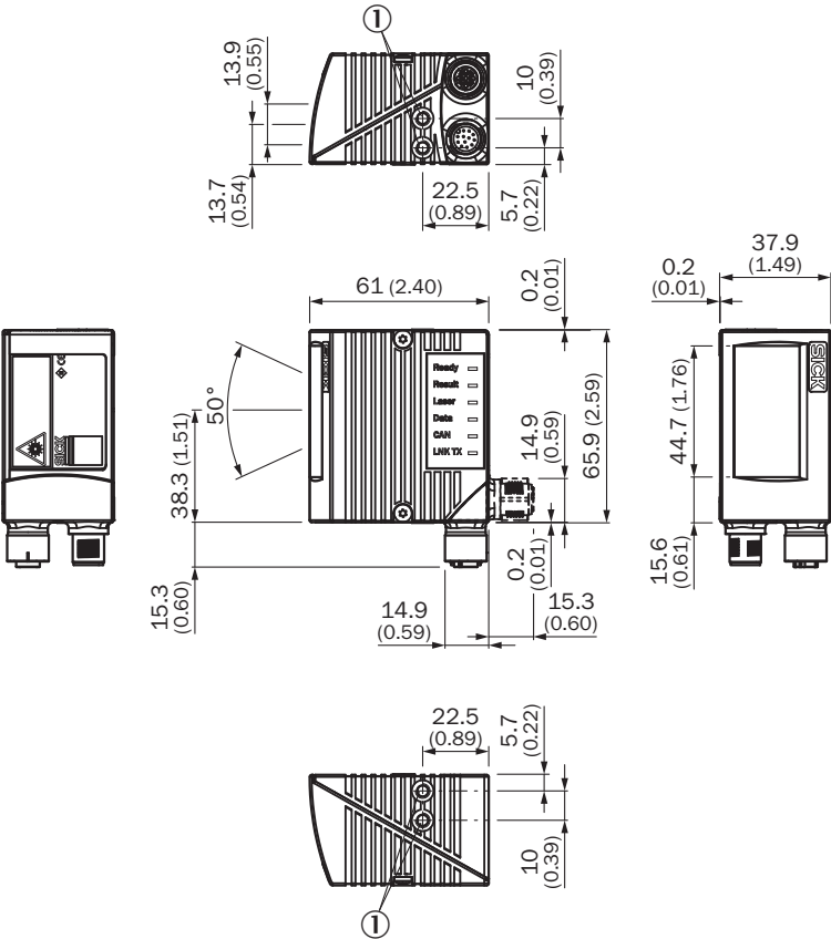
Dimensional drawing CLV62x Ethernet, front
