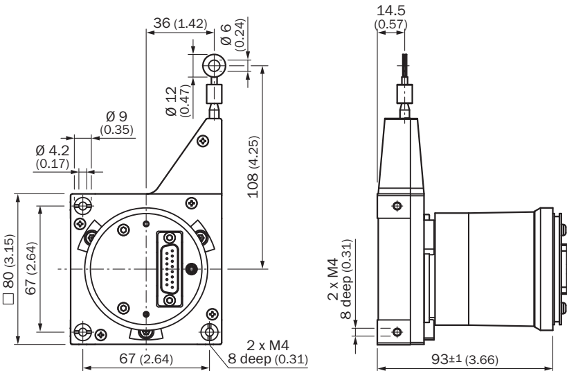
Dimensions in mm (inch)
