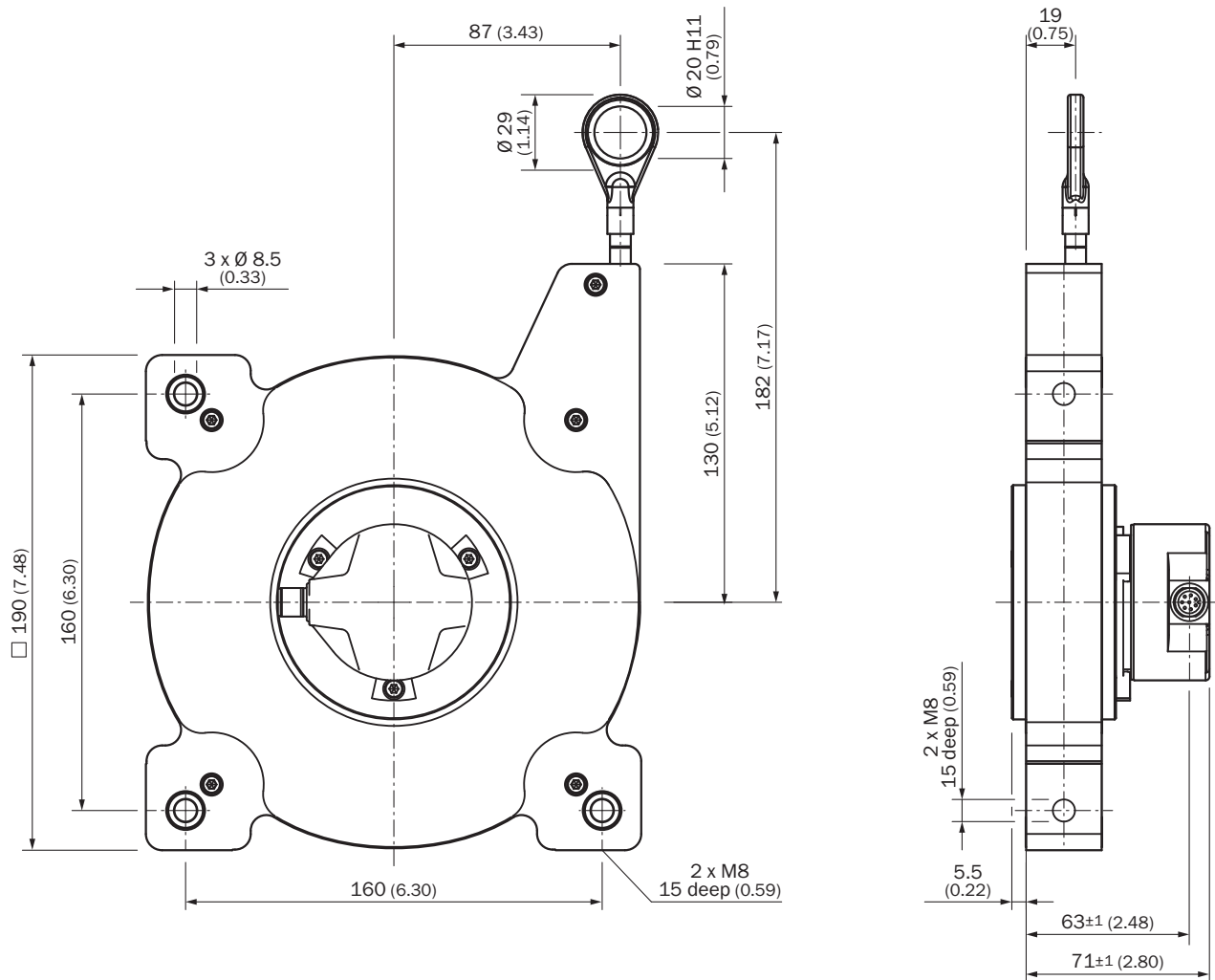
Dimensions in mm (inch)
