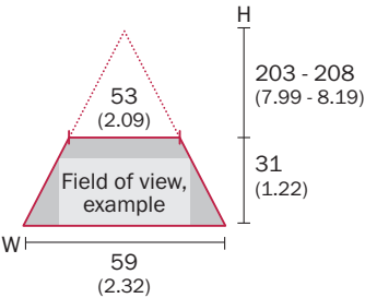
IVC-3D 30 Typ. field of view in mm (inch)
