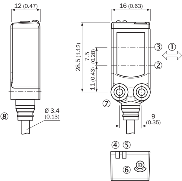
Dimensional drawing WTx4-3, Single teach-in button
