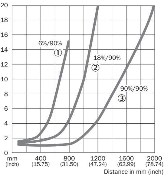
Characteristic curve WTB27-3, PinPoint LED
