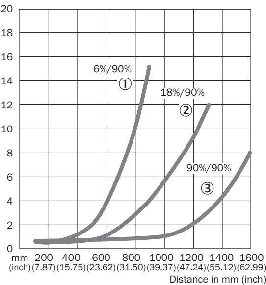
Characteristic curve WTB27-3, infrared
