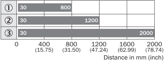
Sensing range diagram WTB27-3, PinPoint LED
