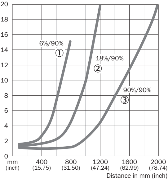
Characteristic curve WTB27-3, PinPoint LED
