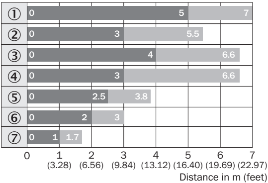
Sensing range diagram WL18-3, WL18-3 Ex
