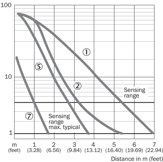
Characteristic curve WL18-3, WL18-3 Ex
