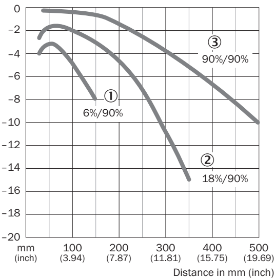
Characteristic curve WTF12-3, 500 mm
