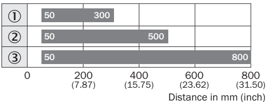
Sensing range diagram WTF12-3, 500 mm
