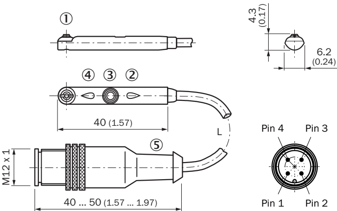
Dimensional drawing Cable with connector M12, with knurled nut
