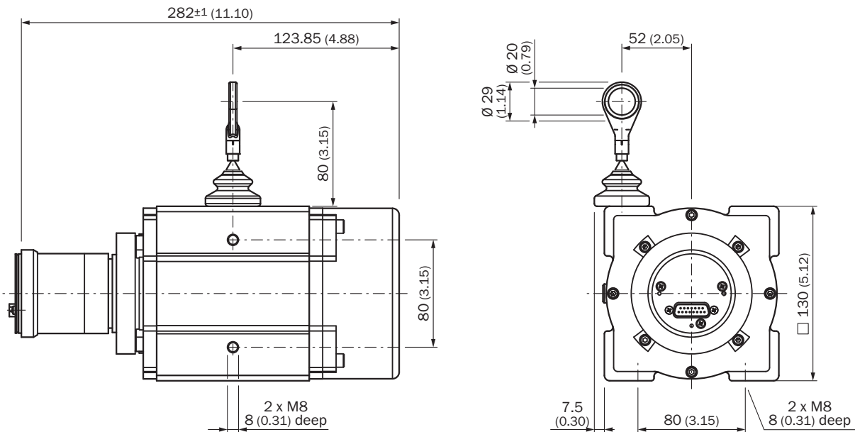
Dimensions in mm (inch)
