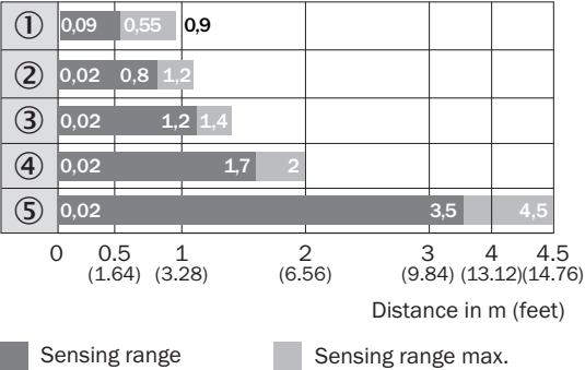
Sensing range diagram WLG4-3 with polarisation filter
