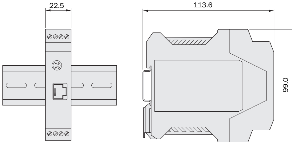
Dimensions in mm (inch)
