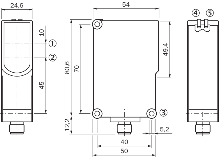
Dimensional drawing WL27-3, WSE27-3
