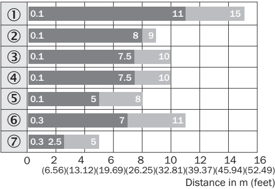
Sensing range diagram WL27-3
