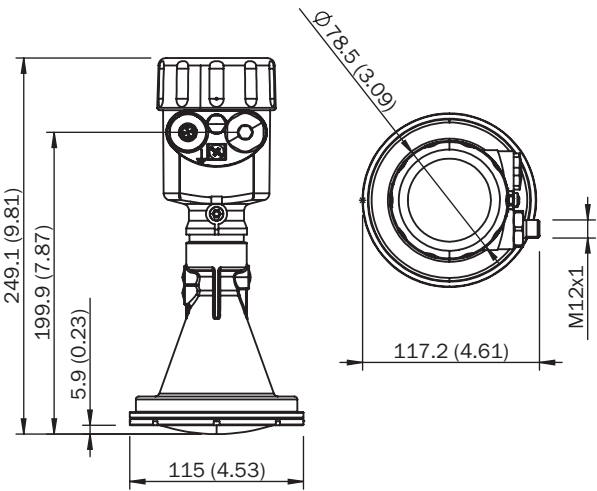
Afmetingen in mm (inch) LFR-xxBXXCBHKKX
