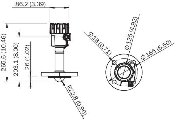
Afmetingen in mm (inch) LFR-xxFFBJ2HAAX
