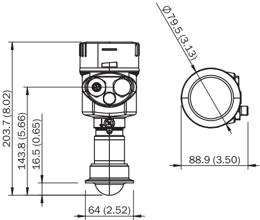
Afmetingen in mm (inch) LFR-xxHCAIBHZAX
