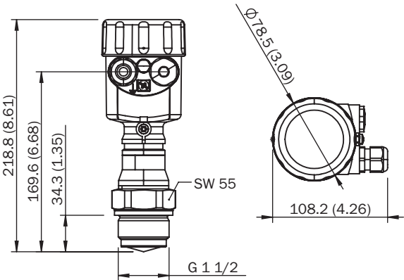
Afmetingen in mm (inch) LFR-xxTTCAMHKAX
