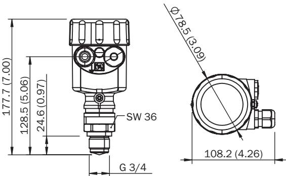
Afmetingen in mm (inch) LFR-xxTTAAMHKAX
