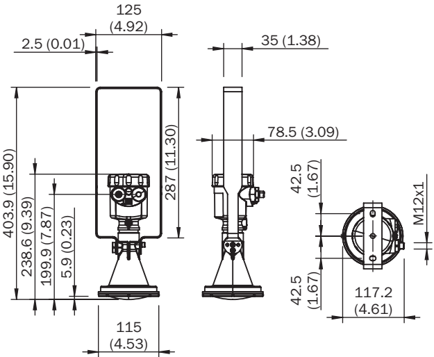
Afmetingen in mm (inch) LFR-xxBXDCBHKXX
