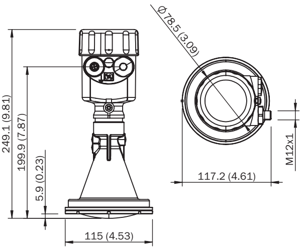
Afmetingen in mm (inch) LFR-xxBXXCBHKXX
