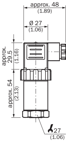
Afmetingen in mm (inch)
