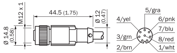
Afmetingen in mm (inch)
