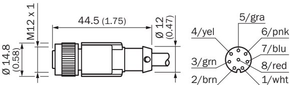
Afmetingen in mm (inch)
