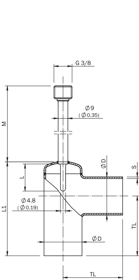
Protection tube with process connenection
