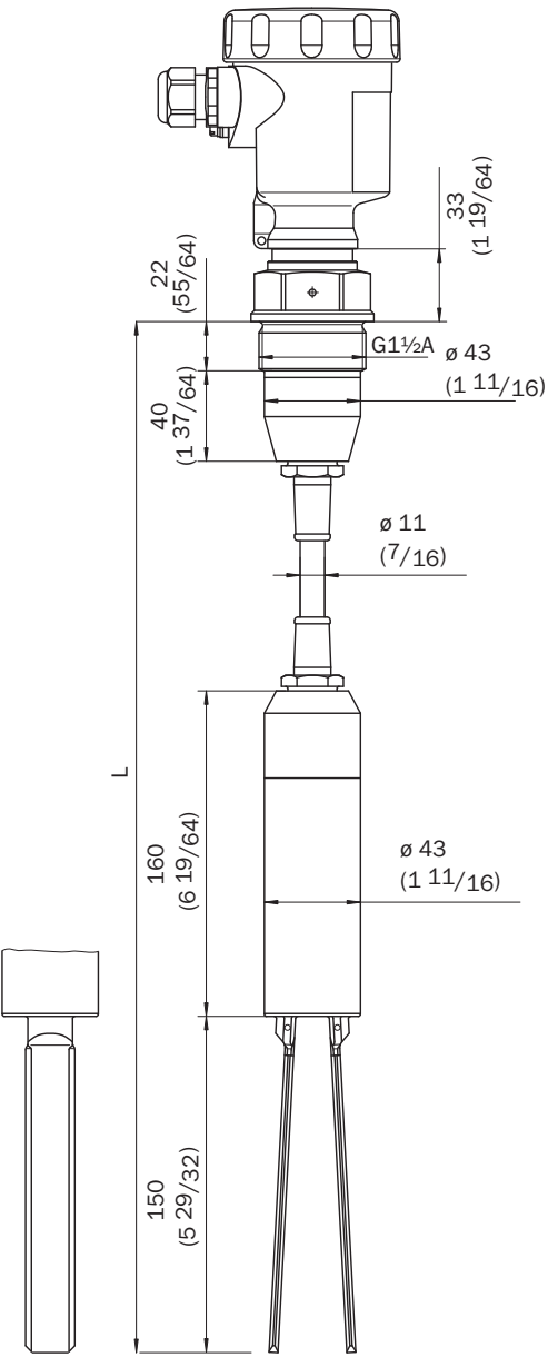
Afmetingen in mm (inch)
