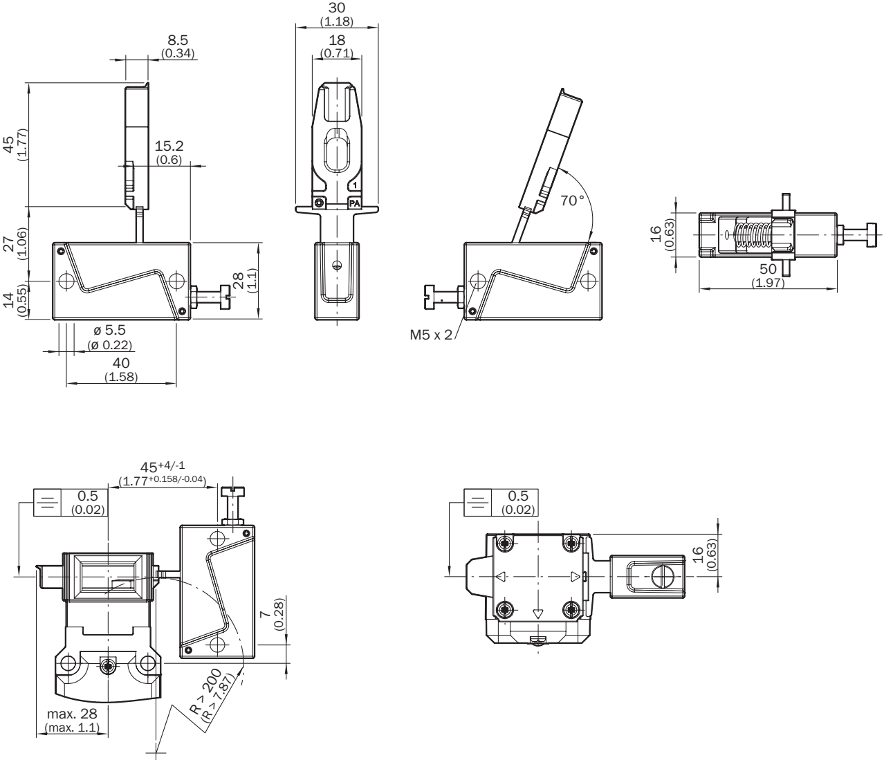
Afmetingen in mm (inch)
