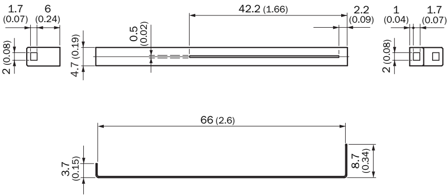
Afmetingen in mm (inch)
