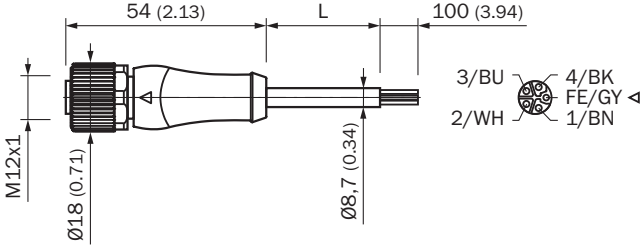
Afmetingen in mm (inch)
