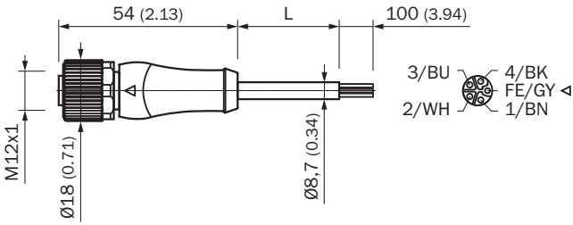
Afmetingen in mm (inch)
