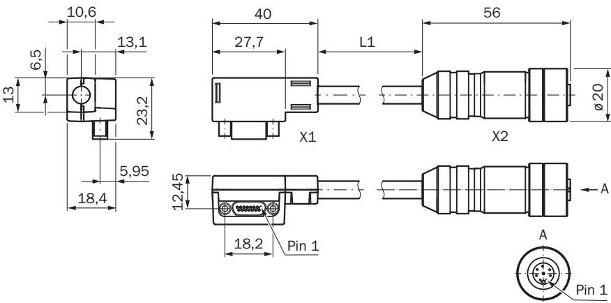
Maattekening (incl. table pin assignment from head A (X1) to head B (X2) for SSI encoder)
