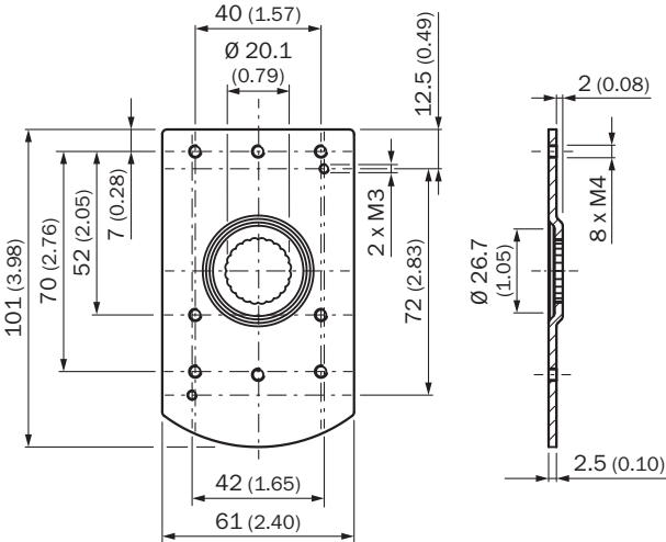
Afmetingen in mm (inch)
