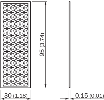
Afmetingen in mm (inch)
