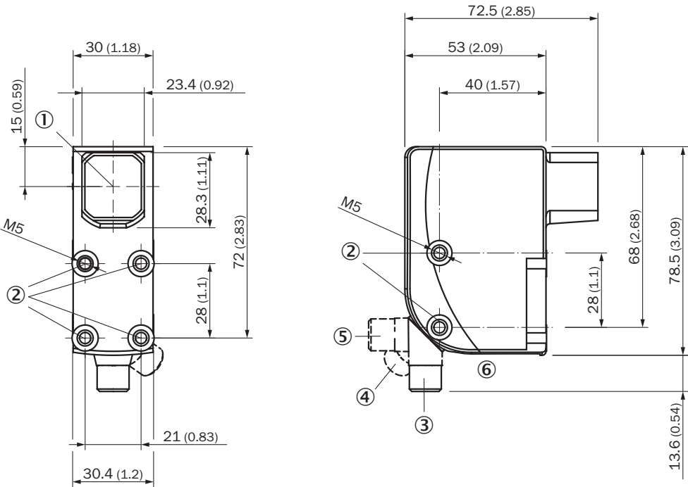
Maattekening Sensing distance from leading edge of lens
