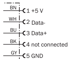
USB Micro-B (Female connector)
