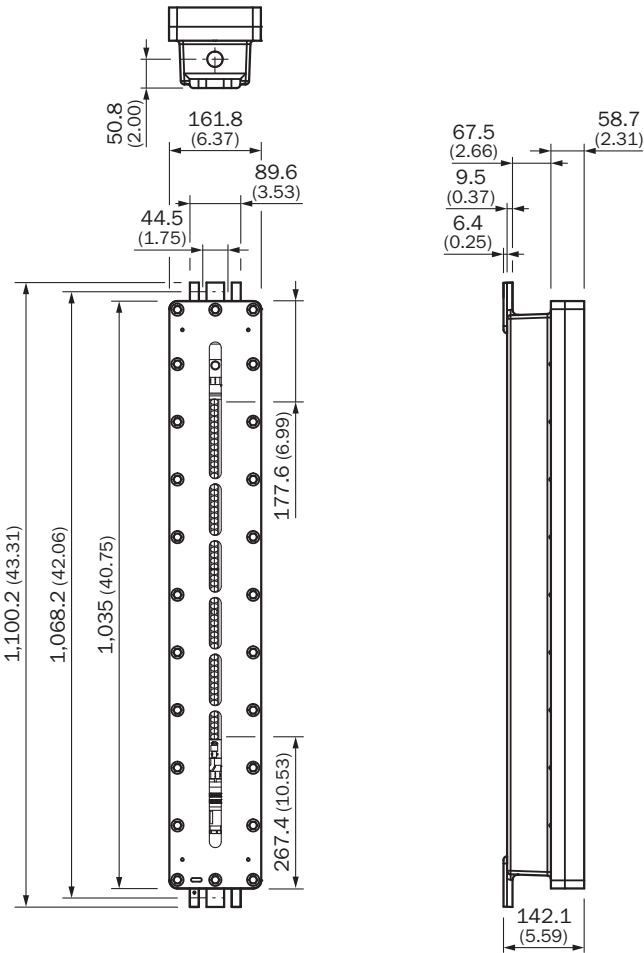
Afmetingen in mm (inch)
