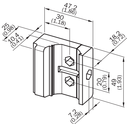
Afmetingen in mm (inch)
