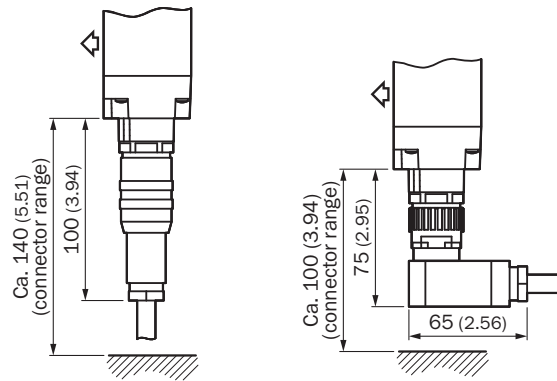
Cable sockets M26 x 11 + FE with crimp contacts
