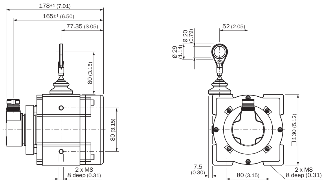
Afmetingen in mm (inch)
