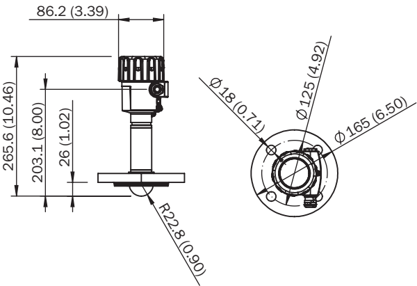
Dimensions en mm (inch) LFR-xxFFBJ2HAAX
