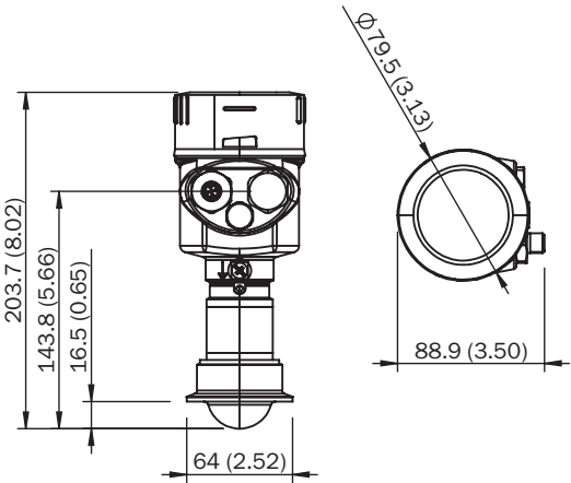
Dimensions en mm (inch) LFR-xxHCAIBHZAX
