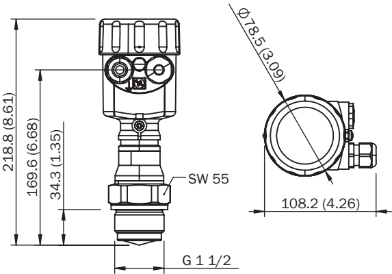
Dimensions en mm (inch) LFR-xxTTCAMHKAX
