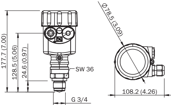
Dimensions en mm (inch) LFR-xxTTAAMHKAX
