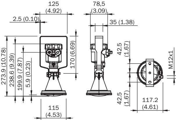
Dimensions en mm (inch) LFR-xxBXCCBHKXX
