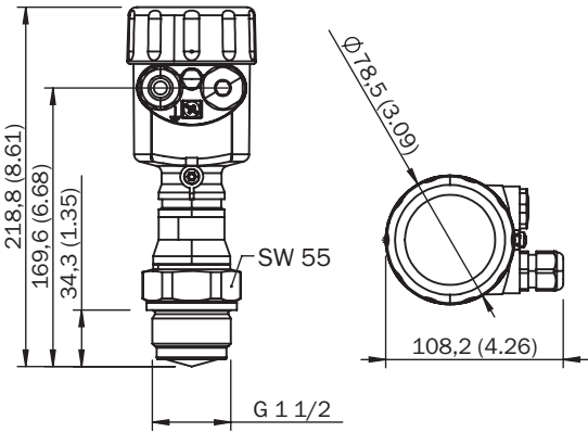
Dimensions en mm (inch) LBR-xxTTCAMHKA
