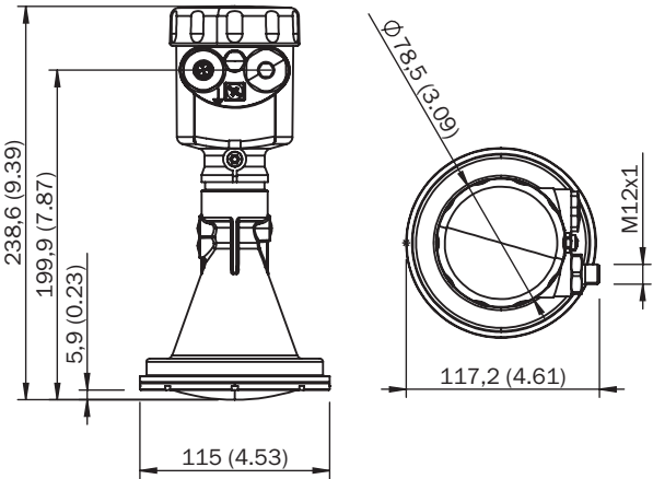
Dimensions en mm (inch) LBR-xxBXXCBHKX
